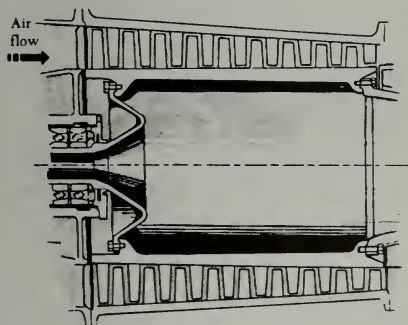
FIGURE 1-41. Drum-type compressor rotor.
